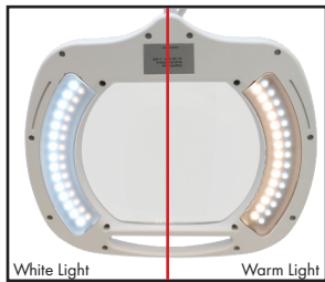
Color Temperature Range: 3500K—6500K Lux rating: 6500LX LED lifespan: Min 20,000 hours
