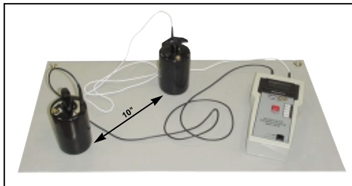
Figure 5. Setting up for Rp testing.
